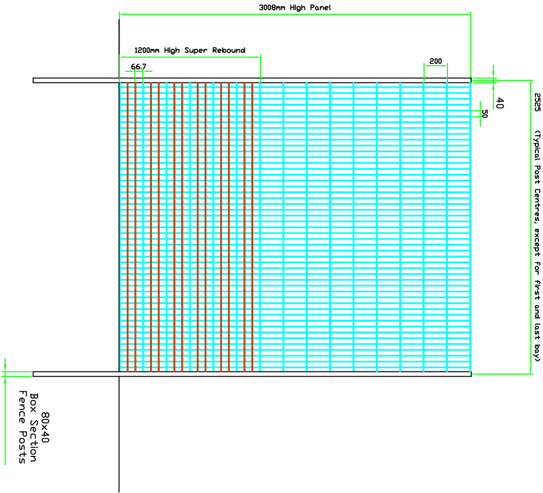
BAY DETAIL
