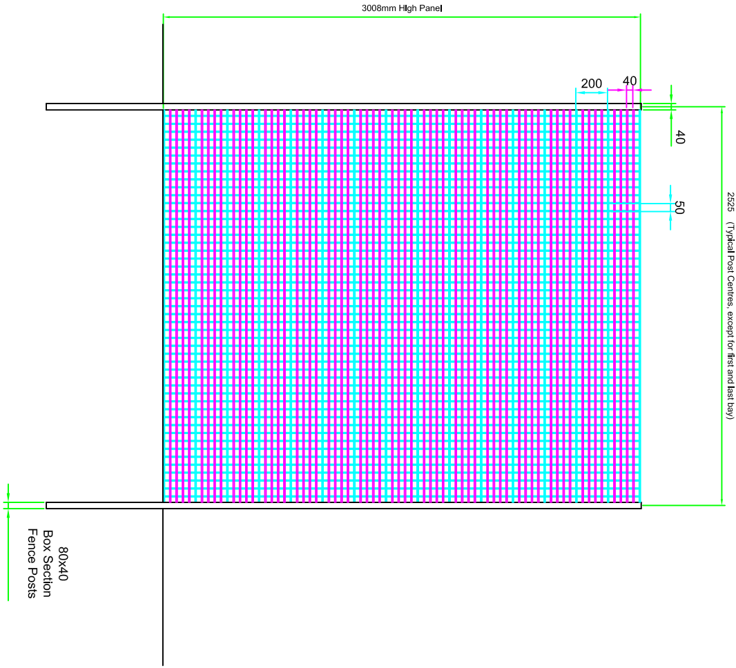
BAY DETAIL
